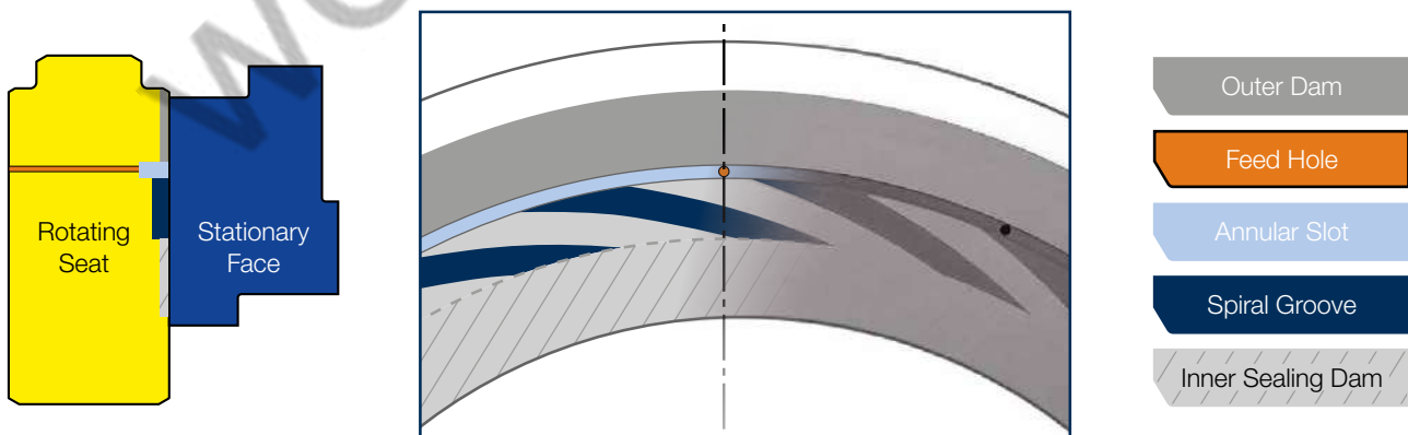
Pictorial view of Pressure Intensifying System
